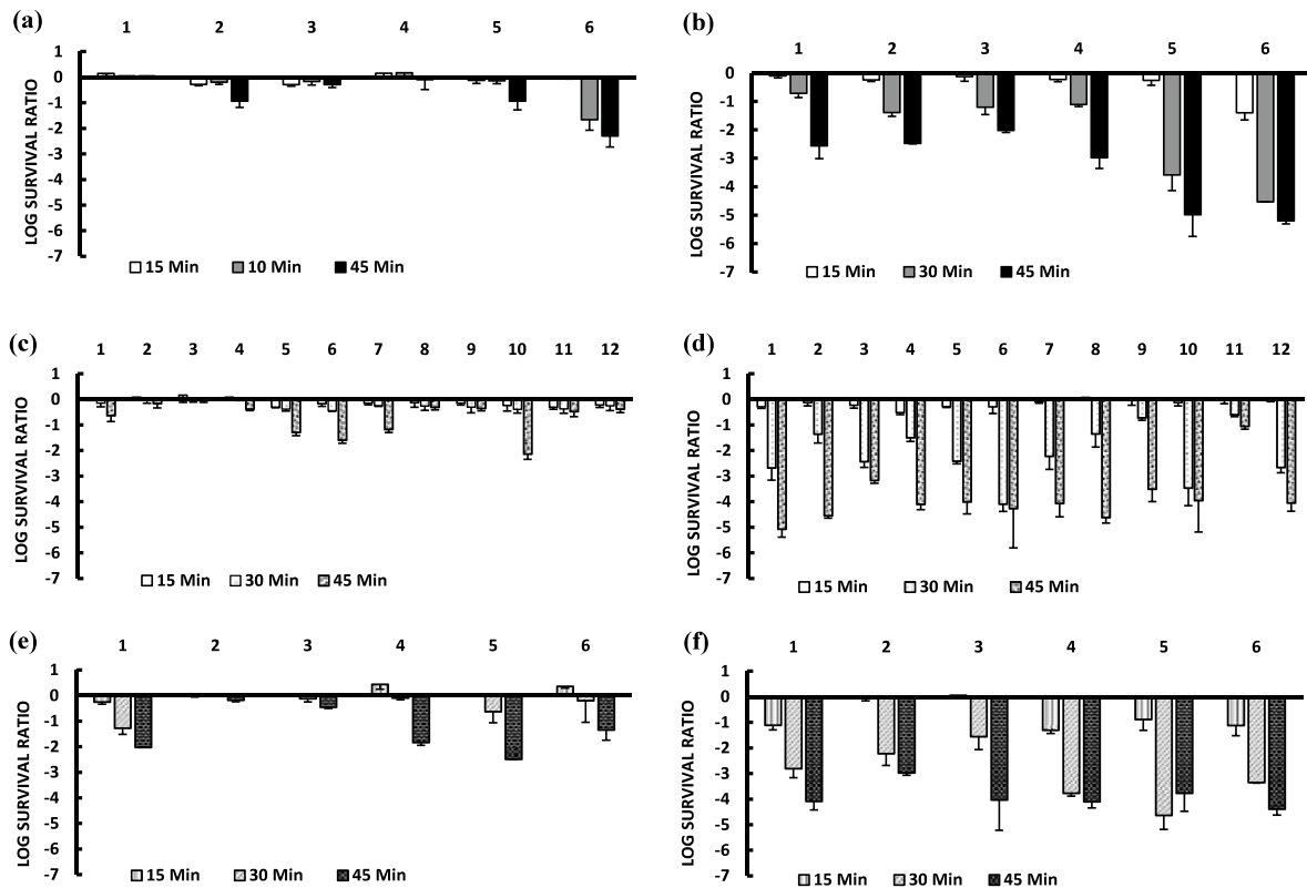
Figure 2. The log survival ratio depends on different output power and irradiation time using the first type of 365 nm UVA-LED. E. coli clinical isolate group in the first line (a and b), ESBL- E. coli clinical isolates group in the second line (c and d), and ESBL- E. coli food isolates group in the third line (e and f). The left side (a, c, e) at the low power (0.23 A) from 15 min (6.23 J/cm 2 ), 30 min (12.47 J/cm 2 ), and 45 min (18.63 J/cm 2 ). The right side (b, d, f) at the high power (0.50 A) from 15 min (13.70 J/cm 2 ), 30 min (27.08 J/cm 2 ), and 45 min (40.76 J/cm 2 ). Values are shown as means \pm SD ( n = 3 , n = number of independent replicates).
